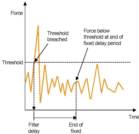
Figure 12a: a random vibration breaches strain gauge force threshold - no trigger issued
