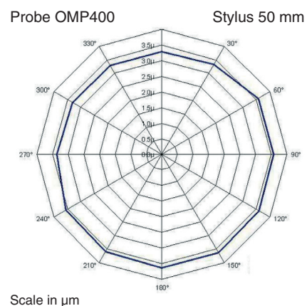
Figure 14: pre-travel variation plot for an OMP400 touch-trigger probe
