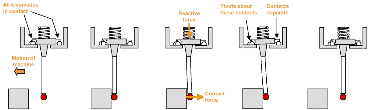
Figure 2: how a kinematic resistive probe generates a trigger
