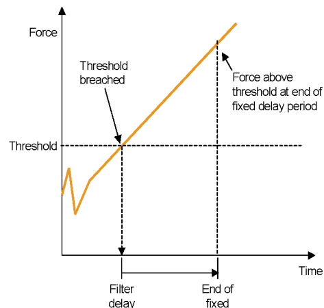
Figure 12b: a persistent force due to a probe trigger breaches strain gauge force - trigger signal is issued at the end of the delay period
