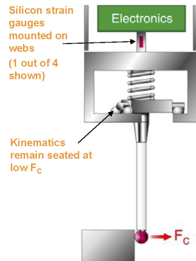
Figure 11: schematic of a strain gauge probe measuring the contact force
