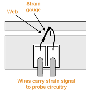
Figure 10: strain gauge mounted to web inside probe
