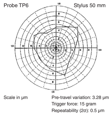
Figure 8: pre-travel variation plot for a TP6 CMM probe
