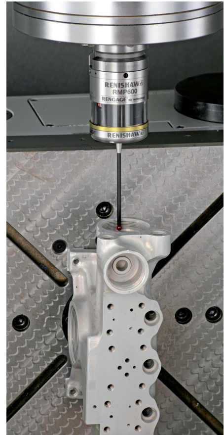
Figure 15: RMP600 strain gauge spindle probe
