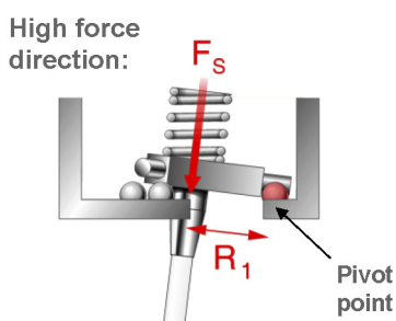
Figure 7a: pivot point is further from stylus centre-line in high force direction
