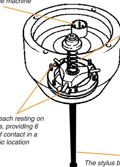
Figure 1: schematic of a kinematic resistive probe
